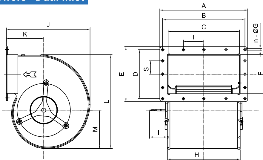
Dimensions (mm)
