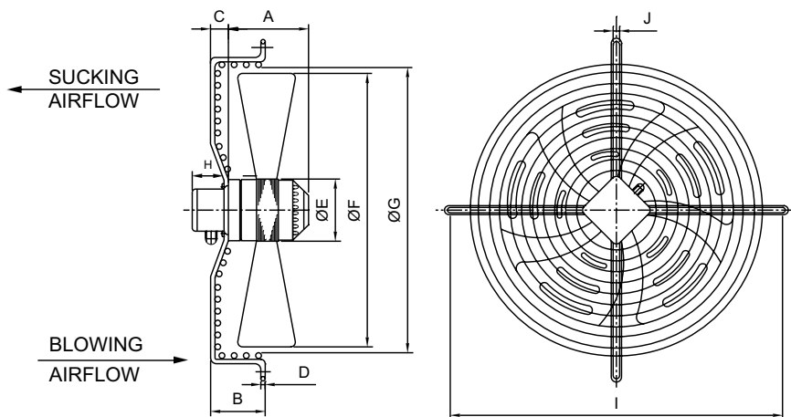
Dimensions (mm)
