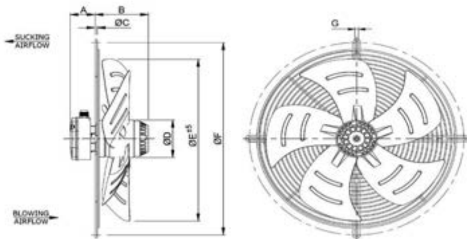
Dimensions (mm)
